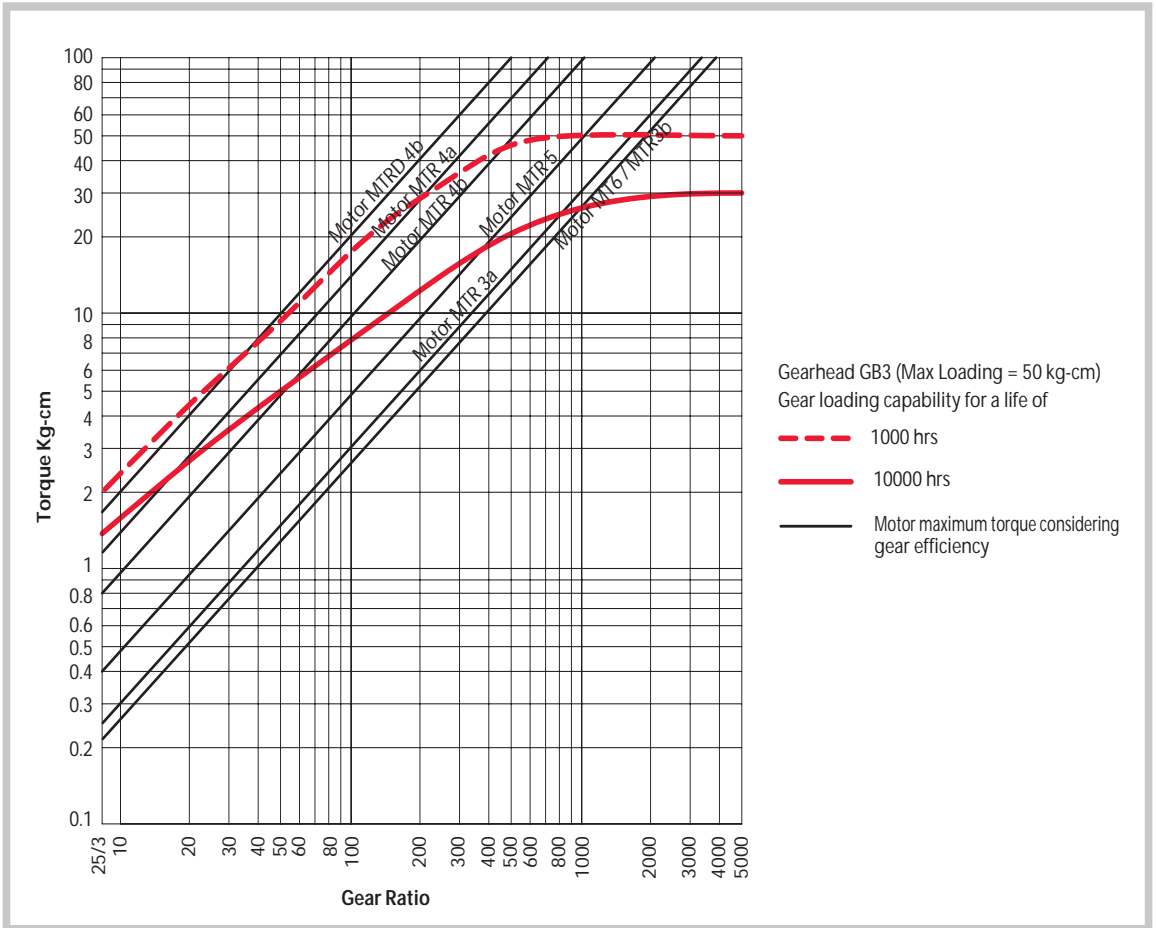
Torque/Transmission ratio/life Graph
